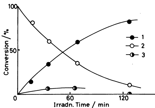
Fig. 2. Time-conversion plots for the direct photolytic isomerization of 2 at 436 nm; [2]=2.5 mM.
